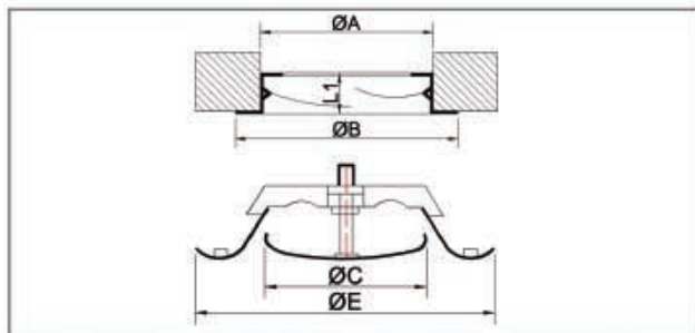
DV-VE Exhaust Valve
